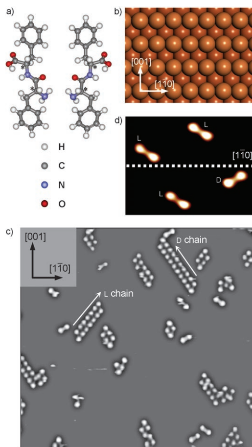
Figure 1. a) Schematic drawing of the L-Phe-L-Phe (right) and D-Phe-D-Phe (left) molecules; the asterisks show the stereocenters. b) Ball model of the Cu(110) surface. c) STM image ( 36 \times 34 nm) of co-adsorbed L-Phe-L-Phe and D-Phe-D-Phe on Cu(110) at room temperature. The arrows indicate the growth direction of the homochiral chains. d) STM image ( 8.3 \times 6.4 nm) of individual di-phenylalanine molecules showing that the two enantiomers are mutual mirror reflections with respect to the plane perpendicular to the surface through the [1\bar{1}0] axis. The color scales are adapted in each image to enhance the molecular contrast.
